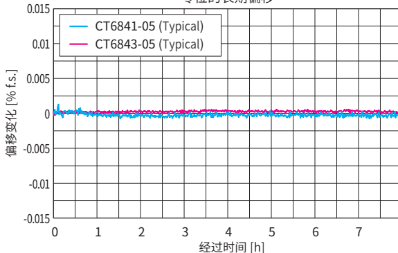
零位的长期偏移
